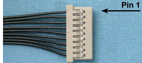
Hirose DF14-09S-1.25C
