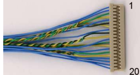
Hirose DF14-20S-1,25C
