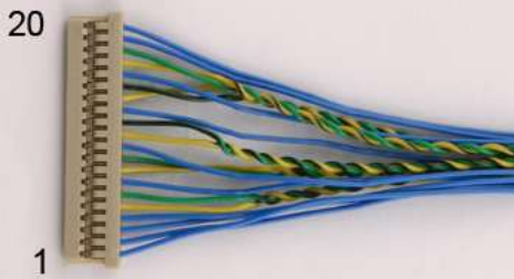
Hirose DF14-20S-1,25C
