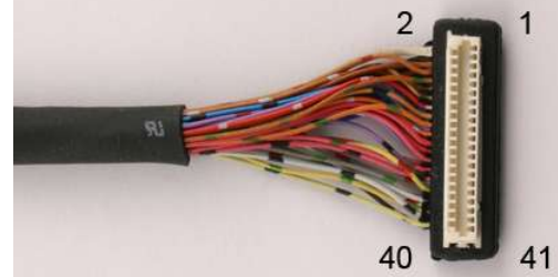
Hirose DF9-41S-1V
