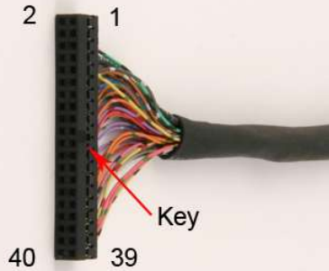
Housing 2 x 20 pitch 2,0 mm
