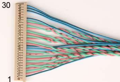
Hirose DF14-30S-1,25C
