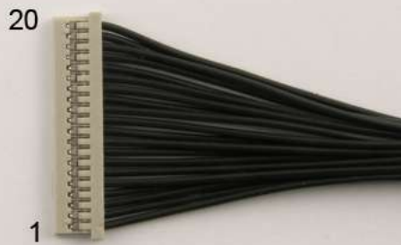
Hirose DF14-20S-1,25C
