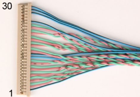
Hirose DF14-30S-1,25C
