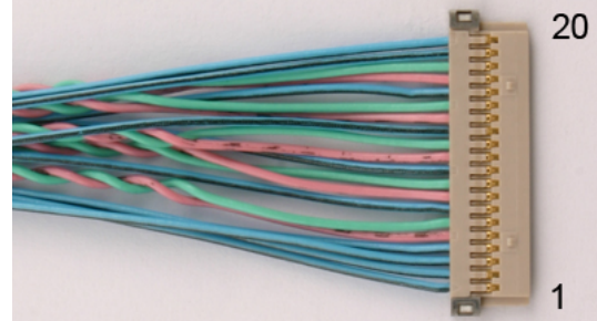
Hirose DF19-20S-1C
