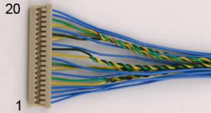
Hirose DF14-20S-1,25C
